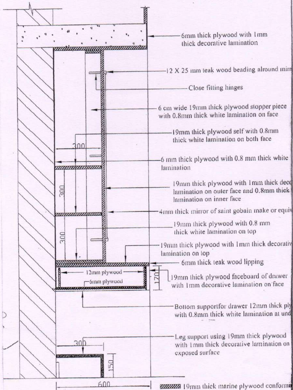
SECTION B-B
